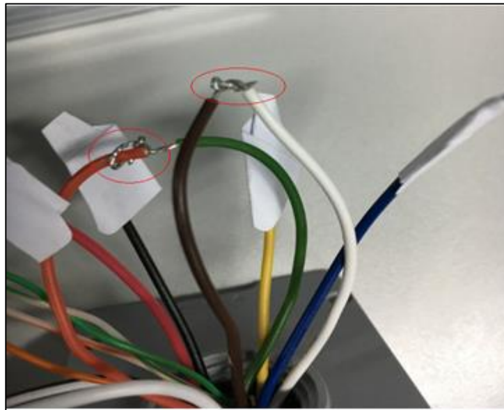
Figure 80: Wiegand Cable Connection
