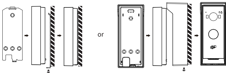
Wall-mounted installation
